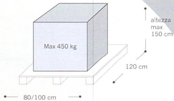
HALF PALLET LIGHT
